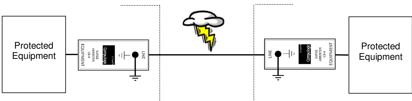
Typical Installation
